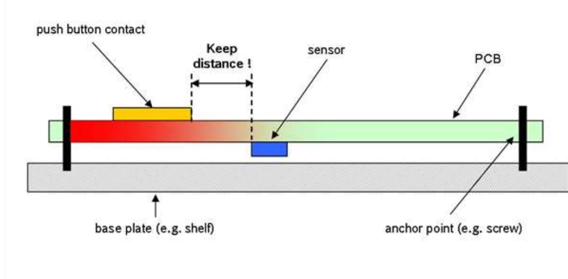
Figure 1: Push-button contacts
