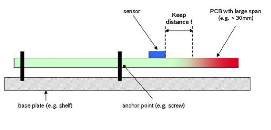
Figure 6: Vibrating PCB
