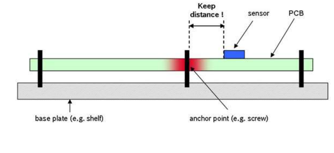
Figure 5: Distance to PCB anchor points
